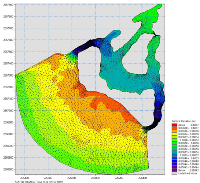
Numerical Model of Proposed Lagoon
